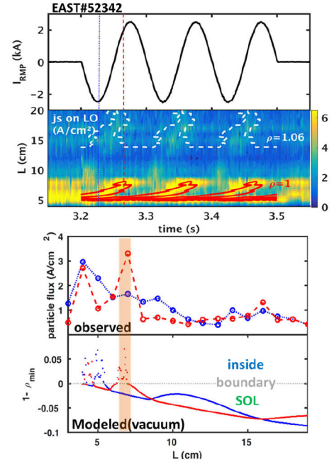
Figure 2: The particle flux temporal evolution with the rigid rotating RMP field is consistent with the numerical modeling of magnetic footprint.
